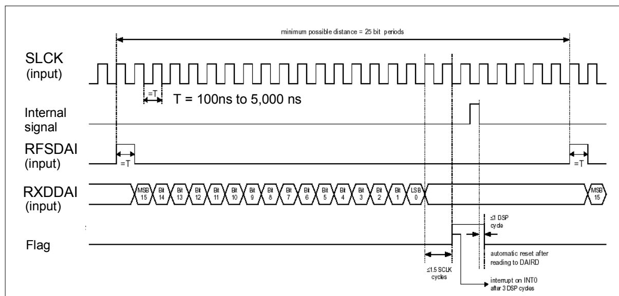
Figure 18: DAI timing on transmit path
